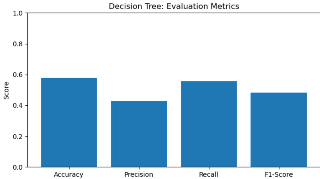
Figure 3. Decision Tree Performance Metrics
