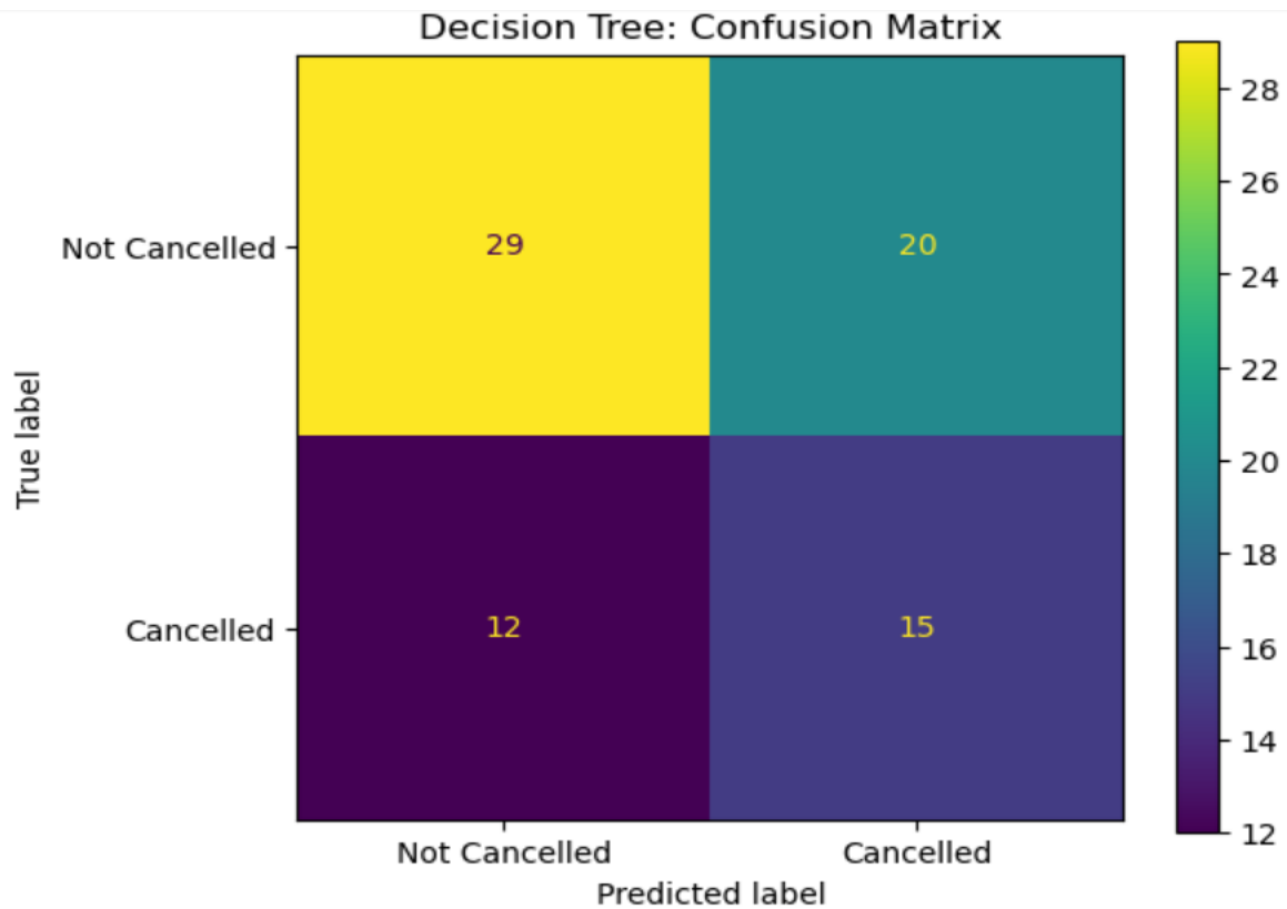
Figure 2. Decision Tree Confusion Matrix
