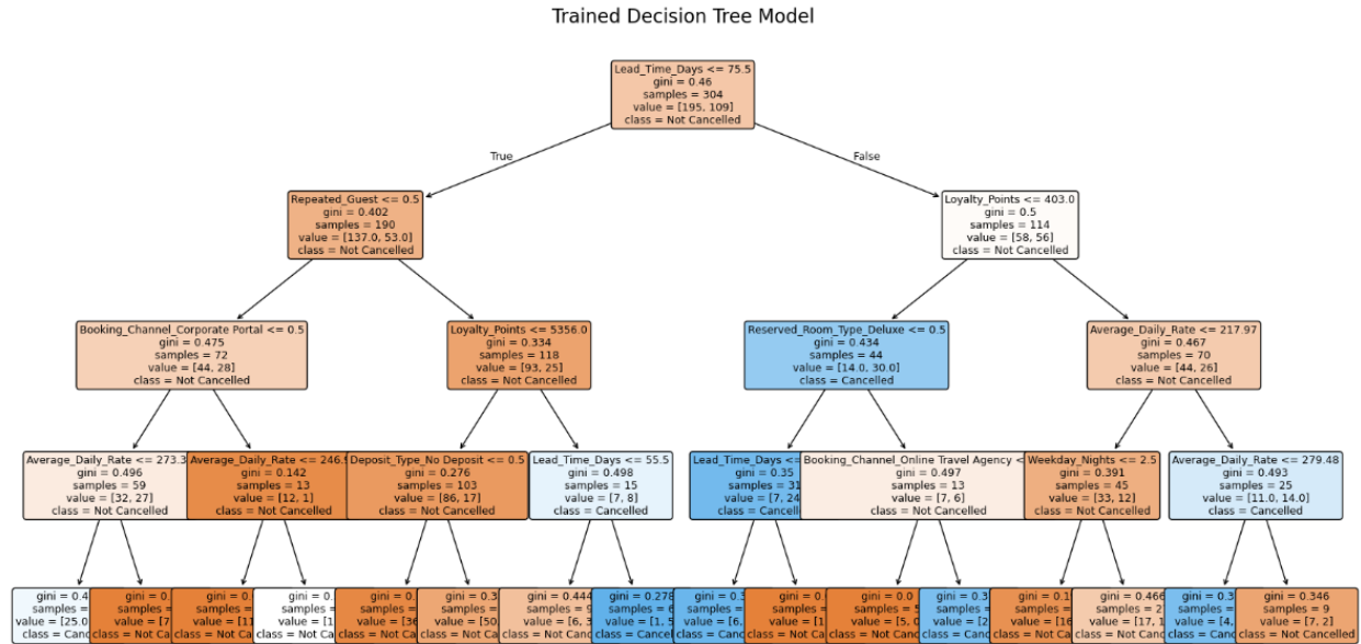
Figure 1. Decision Tree Visualization
